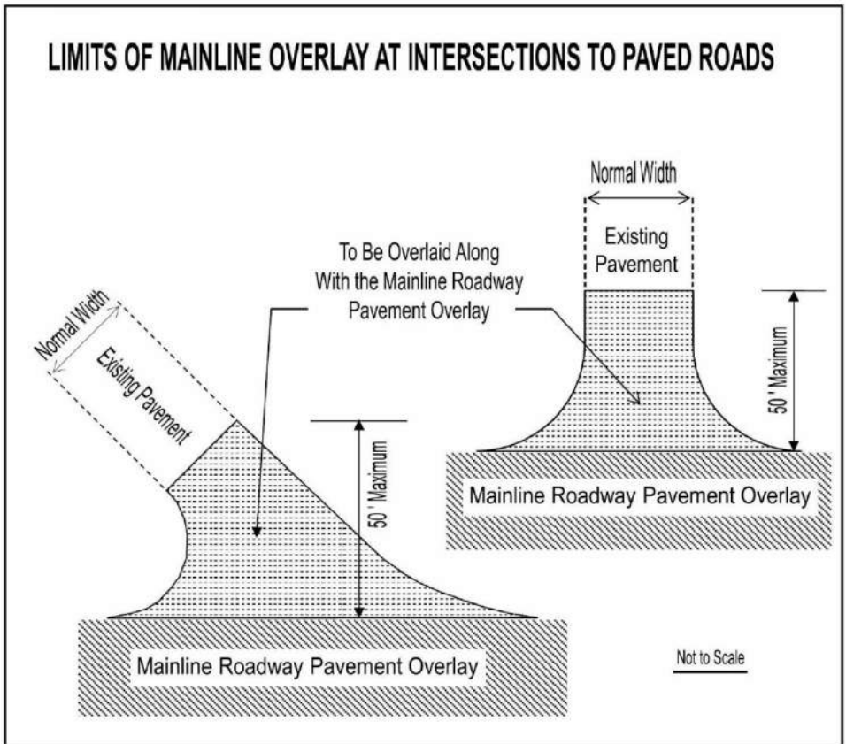
FIGURE III-10 Limits of Mainline Overlay at Intersections to Paved Roads
